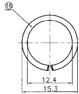
SPRINGWASHER 1 PCS
