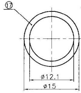
WASHER 1PCS
